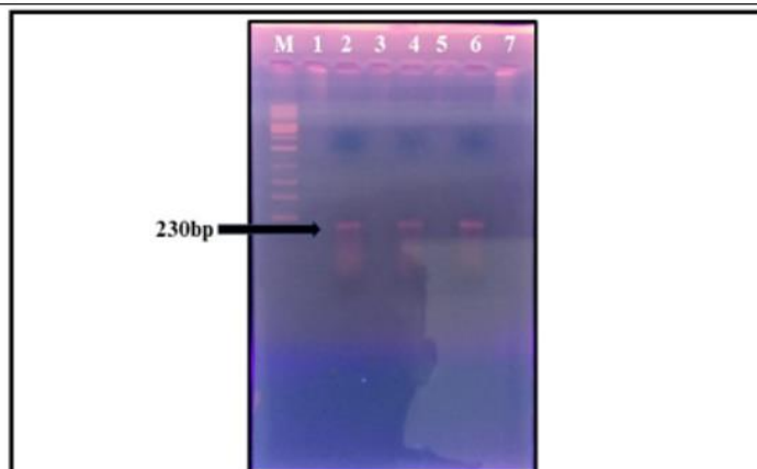
Fig 5: PCR amplification of species specific gene of S. aureus from S. aureus culture. Amplification of species specific gene of S. aureus at three different annealing temperature produced desired bands of size 230bp when run on 1.5% agarose gel. (Lane M: 1kb DNA ladder of GelPilot, Lane 2: Product of 52°C, Lane 4: Product of 54°C, Lane 6: Product of 56°C annealing temperature
