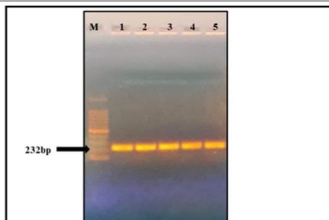
Fig 4: PCR amplification of species specific gene of P. aeruginosa from P. aeruginosa culture. Amplification of species specific gene of P. aeruginosa at different annealing temperature produced desired bands of size 232bp when run on 1.5% agarose gel. (Lane M: 1kb DNA ladder of GelPilot, Lane 1: Product of 57°C, Lane 2: Product of 59°C, Lane 3: Product of 61°C, Lane 4: Product of 63°C, Lane 5: Product of 65°C annealing temperature.
