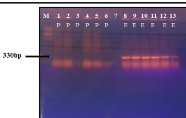
Fig 3: PCR amplification of species specific gene sequence of topoisomerase A of E.coli from E.coli and P.aeruginosa culture. Amplification of topoisomerase A of E.coli using E.coli culture at six different annealing temperatures produced bands of size 330bp when run on 1.5% agarose gel. However, no bands were observed for P.aeruginosa culture in any of the annealing temperature. (Lane M: 1kb DNA ladder of GelPilot, Lane 1: 56°C, Lane 2: 58°C, Lane 3: 60°C, Lane 4: 62°C, Lane 5: 64°C, Lane 6: 66°C annealing temperature products using P.aeruginosa culture and Lane 8: 56°C, Lane 9: 58°C, Lane 10: 60°C, Lane 11: 62°C, Lane 12: 64°C, Lane 13: 66°C annealing temperature products using E.coli culture.
