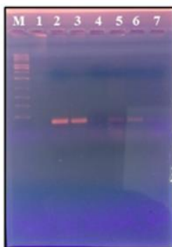
Fig 8: PCR amplification of species specific eap gene of S.aureus using S. aureus , P.aeruginosa and E.coli culture as template. Amplification of species specific eap of S.aureus from S.aureus , P. aeruginosa , E.coli cultures at 56°C annealing temperature produced desired bands when run on 1.5% agarose gel. (Lane M: 1Kp DNA ladder of NEB, Lane 1, 2: using S.aureus culture, Lane 3,4 P. aeruginosa culture and Lane 5, 6: E.coli , culture as template.
